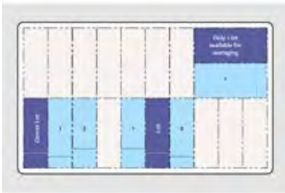
FIGURE 7-H: SETBACK AVERAGING
