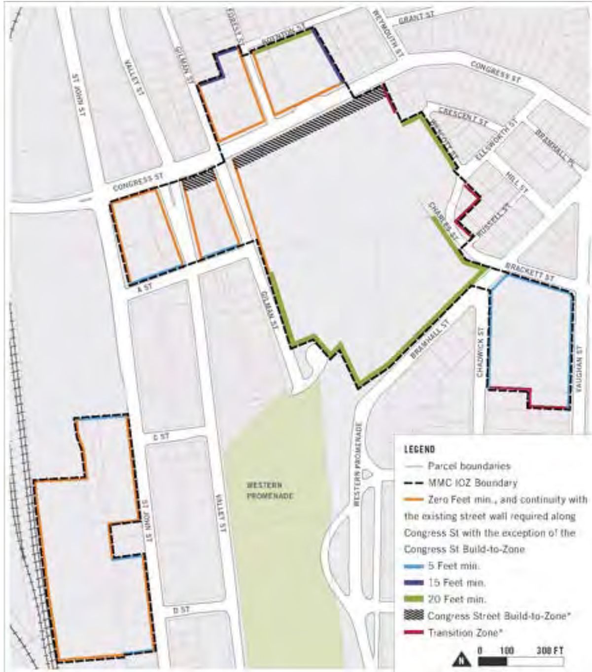
FIGURE 8-E: MINIMUM SETBACKS
