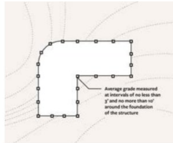
FIGURE 7-D: AVERAGE GRADE
