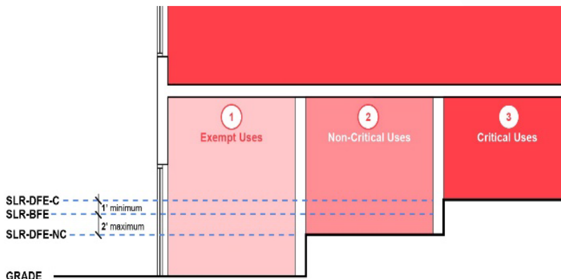
FIGURE 8-A: CFROZ USE CLASSIFICATIONS AND DESIGN FLOOD ELEVATION
