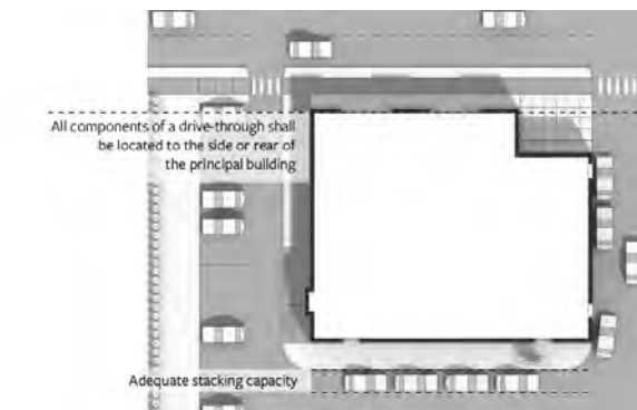
FIGURE 6-A: DRIVE-THROUGH SITING
