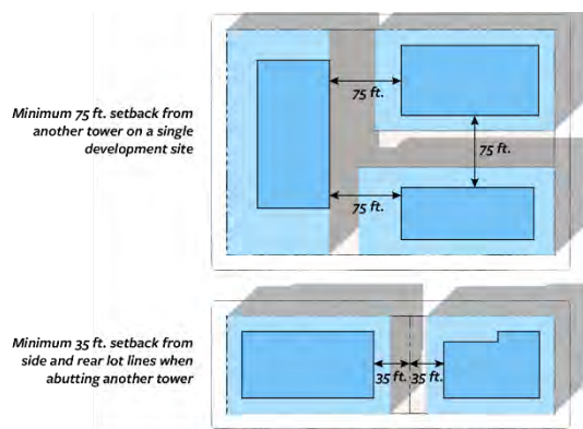
FIGURE 7-L: TOWER SEPARATION
