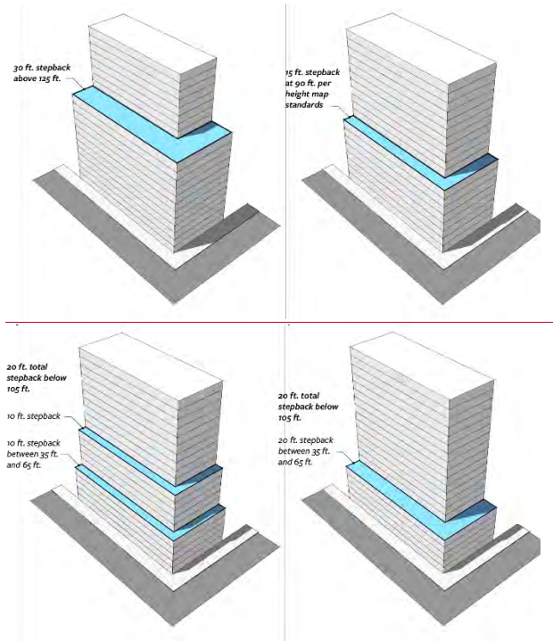
FIGURE 7-J: TOWER STEPBACK
