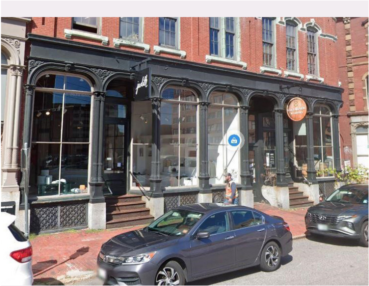
The Rackleff Block (1867, 131 Middle Street) takes advantage of cast iron’s the structural capacity mass producability to create tall, transparent storefronts trimmed out in cost-effective decorative elements such as the ornate column capitols and arched details.
