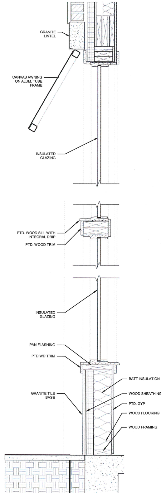
4 | STOREFRONT SECTION 1 1/2" = 1'-0"
