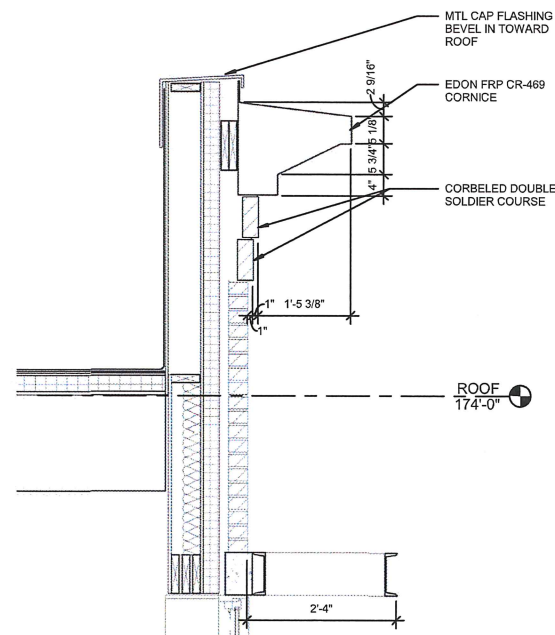
4 | CORNICE DETAIL 3/4" = 1'-0"
