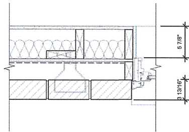
3 | PLAN DETAIL AT WINDOW 1 1/2" = 1'-0"
