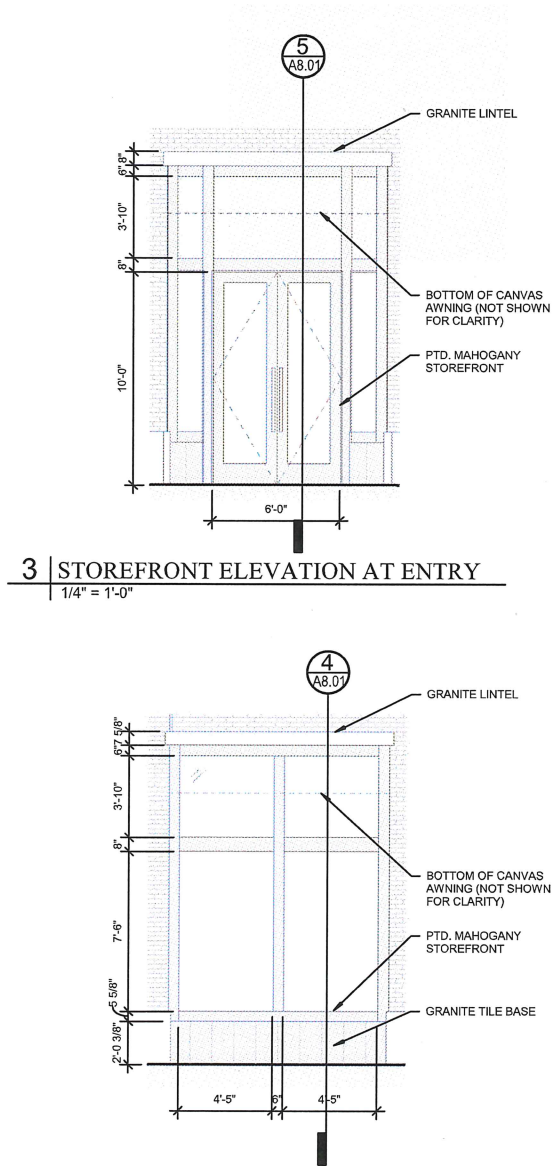
2 | STOREFRONT ELEVATION 1/4" = 1'-0"
