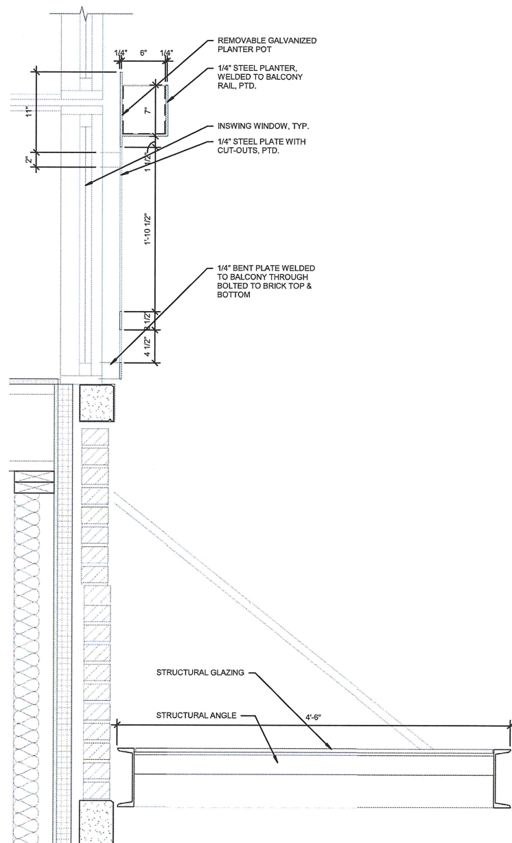
6 | JULIETTE BALCONY DETAIL 1 1/2" = 1'-0"
