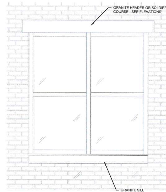
2 | TYPICAL WINDOW ELEVATION 3/4" = 1'-0"
