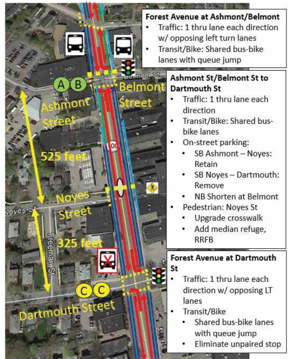
Figure 79. Ashmont Street/Belmont Street to Dartmouth Street – Alternative 2
