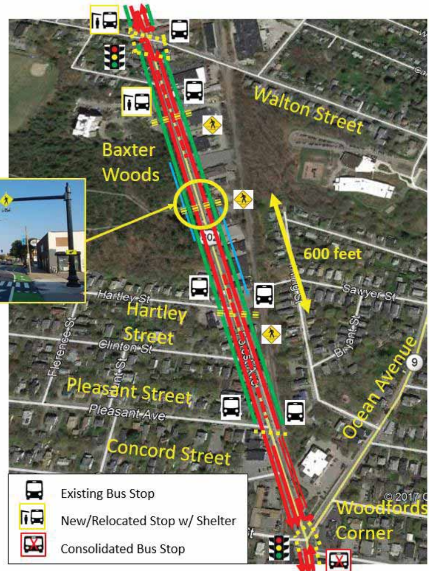
Figure 73. Walton Street to Woodfords Corner — Improvements Evaluated
