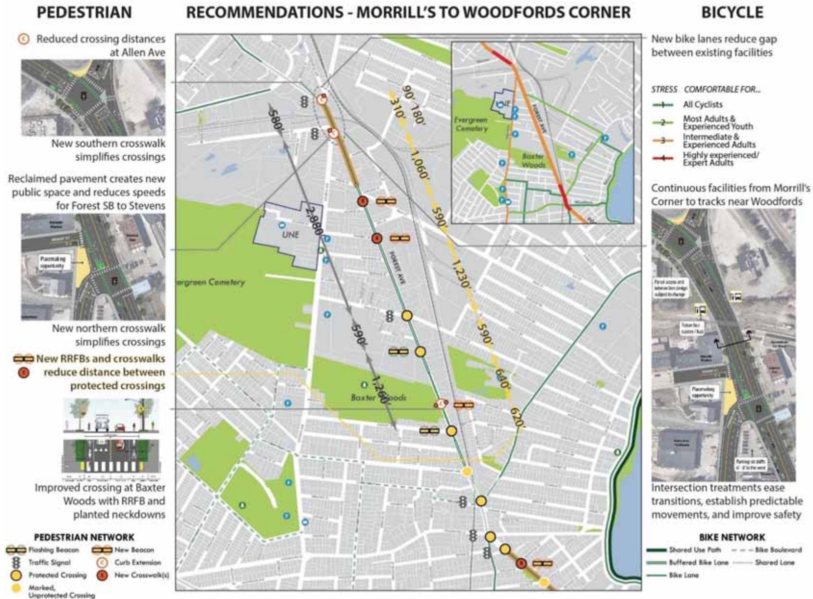
Figure 113. Recommended Pedestrian & Bicycle Improvements – Forest Avenue North
