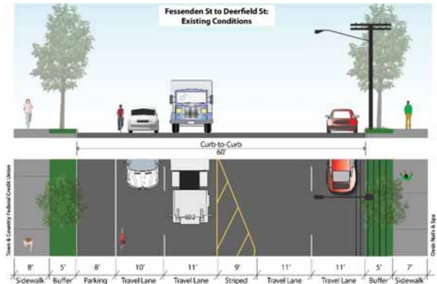
Figure 55. Existing Layout – Forest Avenue from Deerfield Street to Fessenden Street
