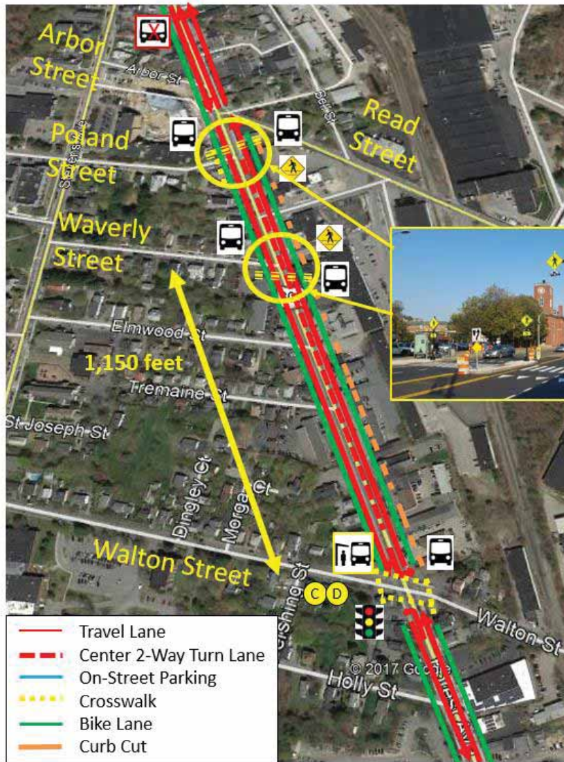
Figure 72. Morrill's Corner to Walton Street — Improvements Evaluated
