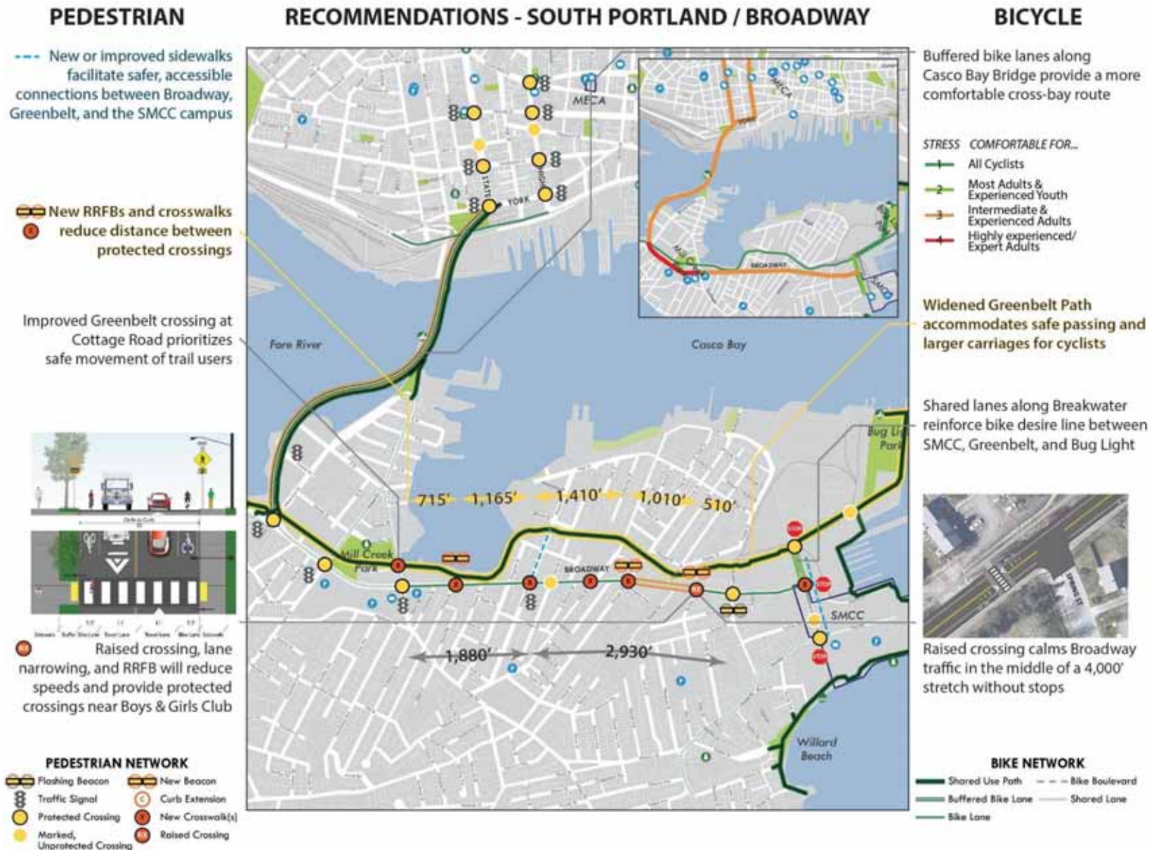
Figure 128. Recommended Pedestrian & Bicycle Improvements – South Portland-Broadway
