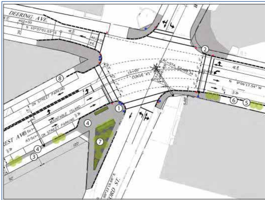
Figure 16. Woodfords Corner Improvement Project, with New Plaza at Forest Avenue/Woodford Street
