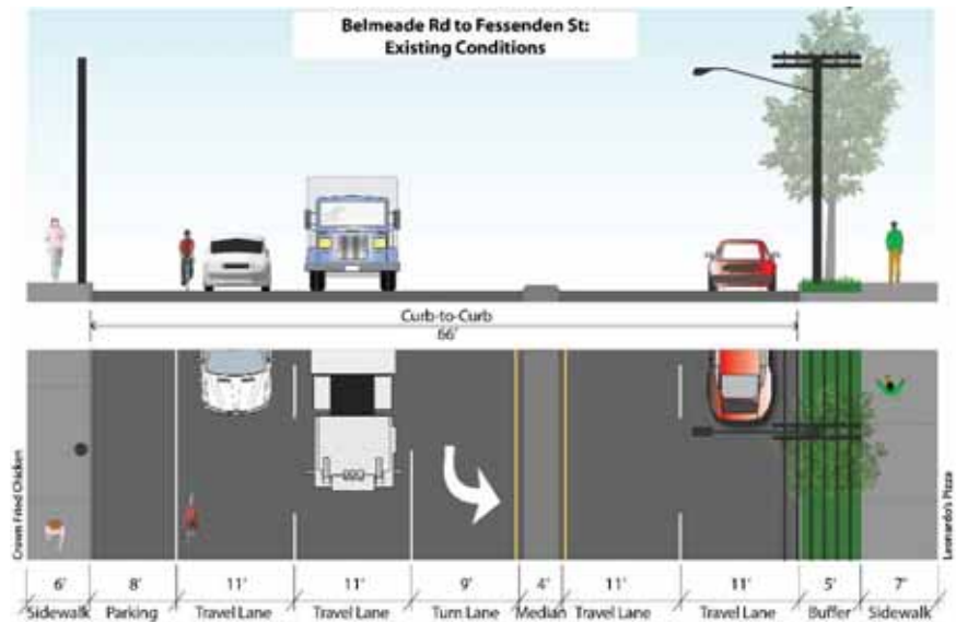
Figure 56. Existing Layout – Forest Avenue from Fessenden Street to Belmeade Road
