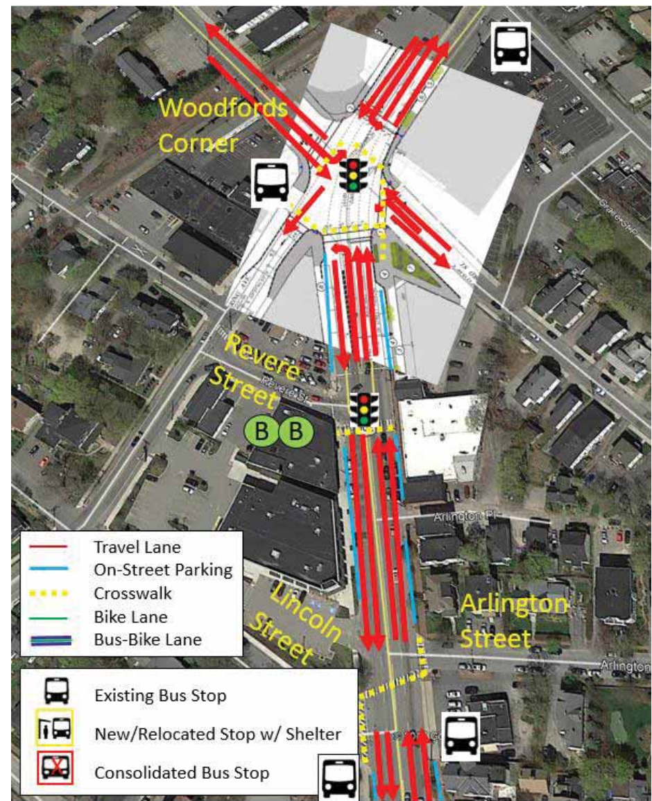
Figure 74. Woodfords Corner to Lincoln Street/Arlington Street – Future No-Build Conditions
