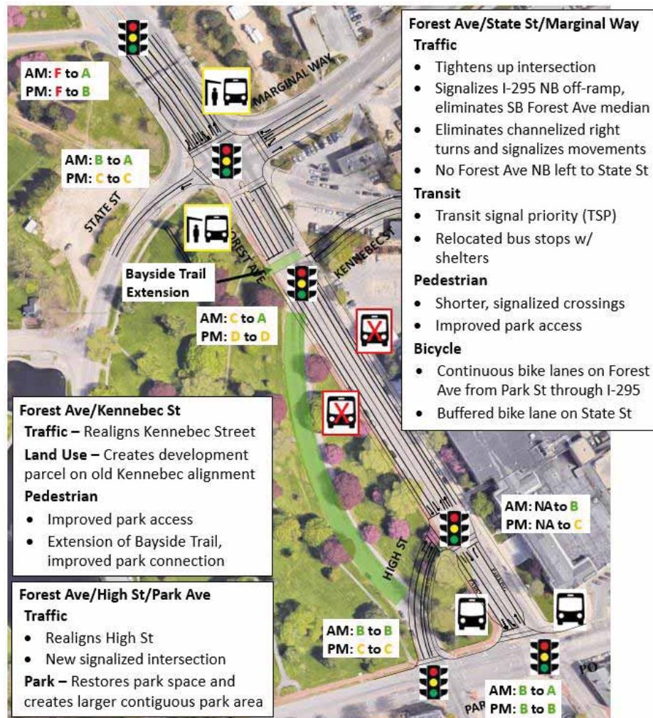
Figure 88. Deering Oaks Park – Alternative 1
