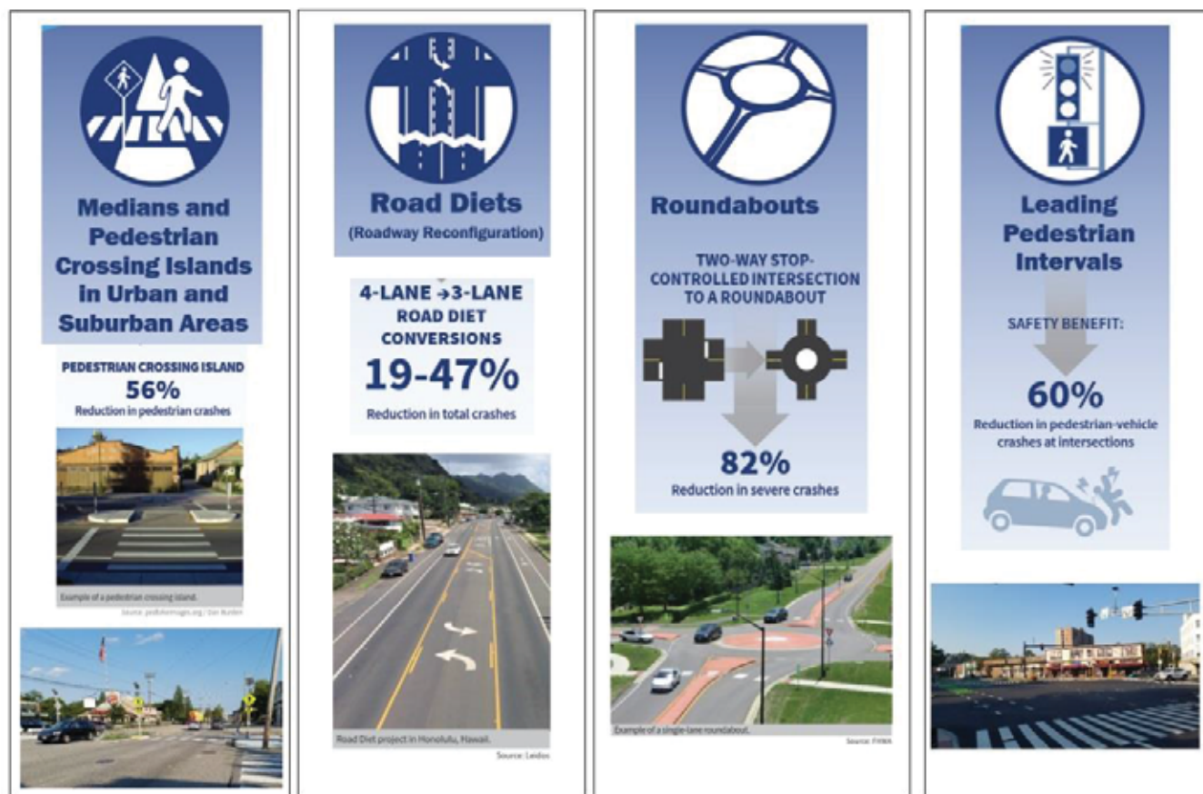
Figure 70. Proven Safety Countermeasures (Source: FHWA)
