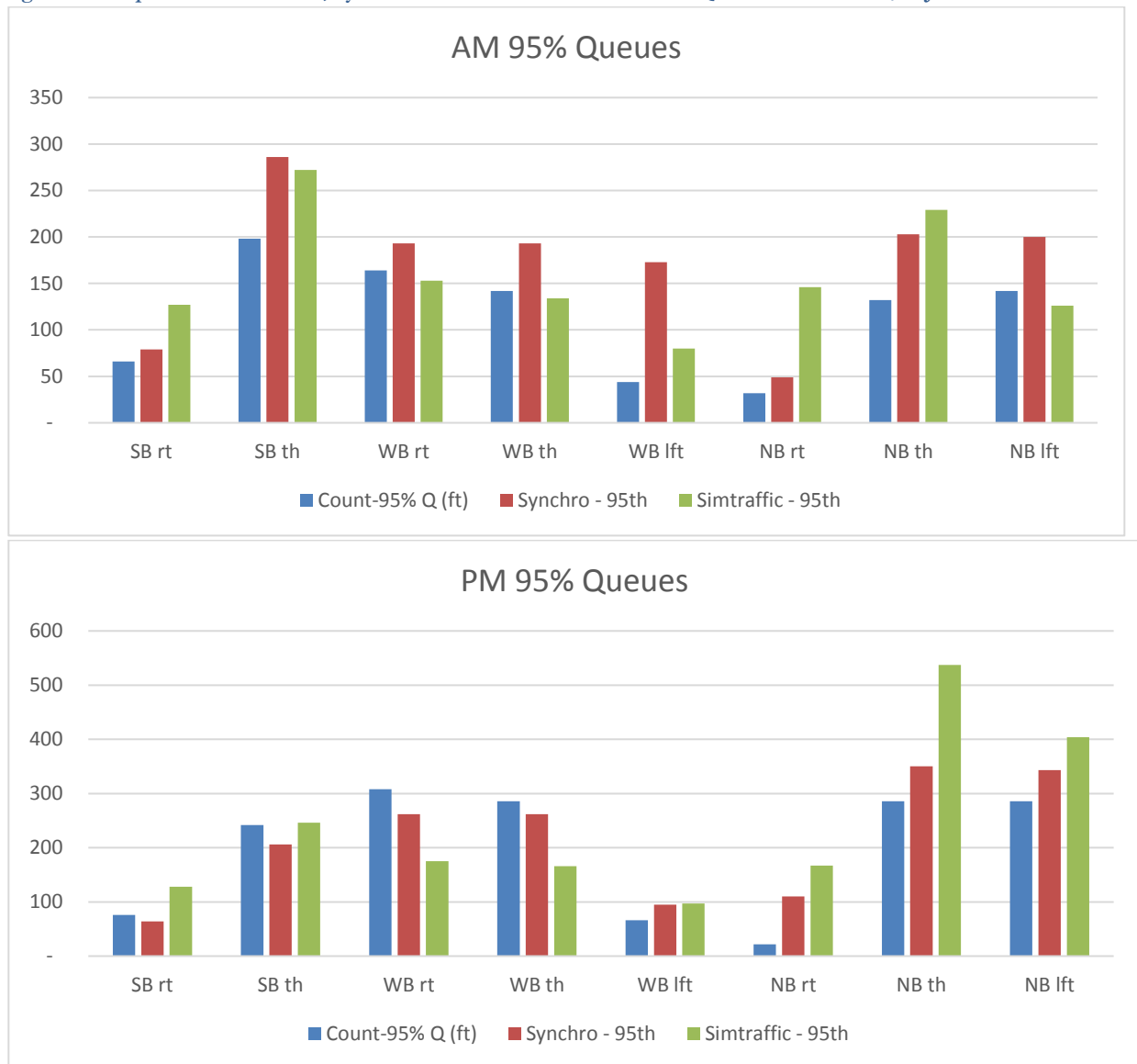
Figure 2: Comparison of Observed, Synchro and SimTraffic 95 th Percentile Queues for Park Ave/St John St Intersection
