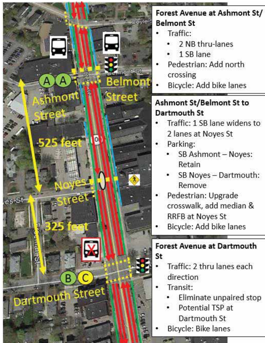
Figure 78. Ashmont Street/Belmont Street to Dartmouth Street – Alternative 1
