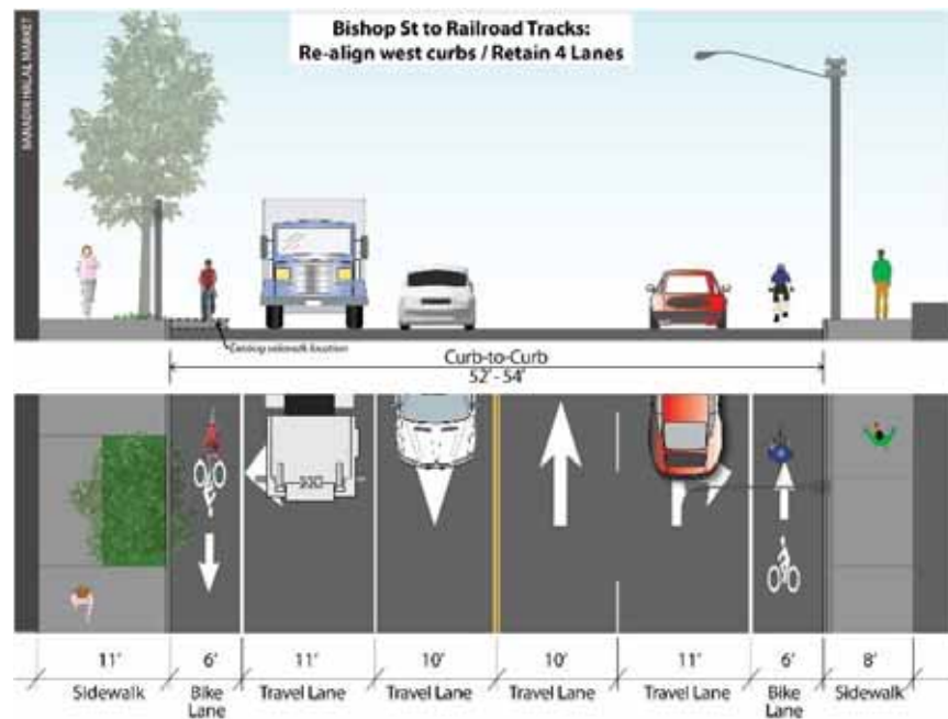
Figure 111. Preferred Alternative — Forest Avenue from Bishop Street to Railroad Tracks
