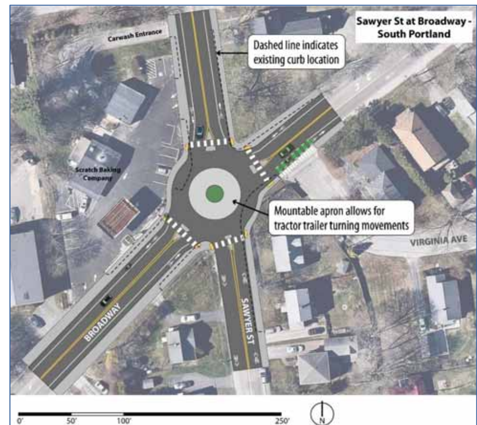
Figure 125. Modern Roundabout at Broadway/Sawyer Street
