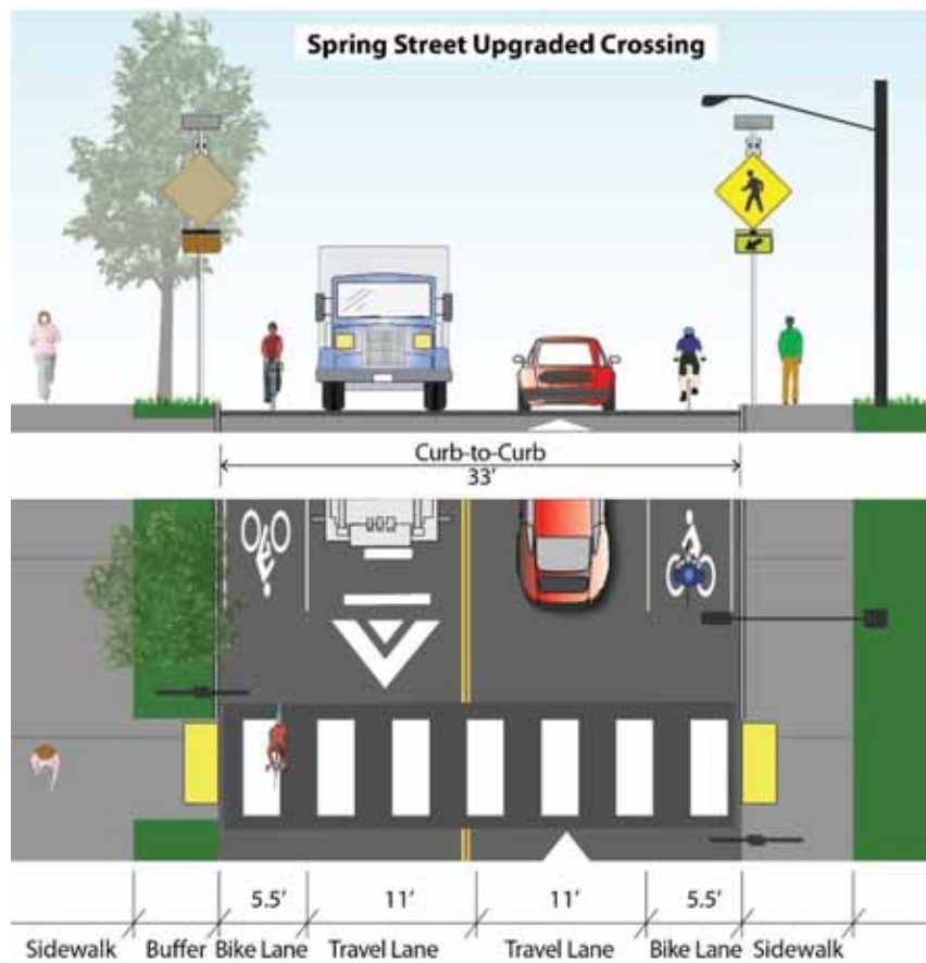
Figure 126. Preferred Alternative — Upgraded Raised Crossing at Broadway and Spring Street (Section View)
