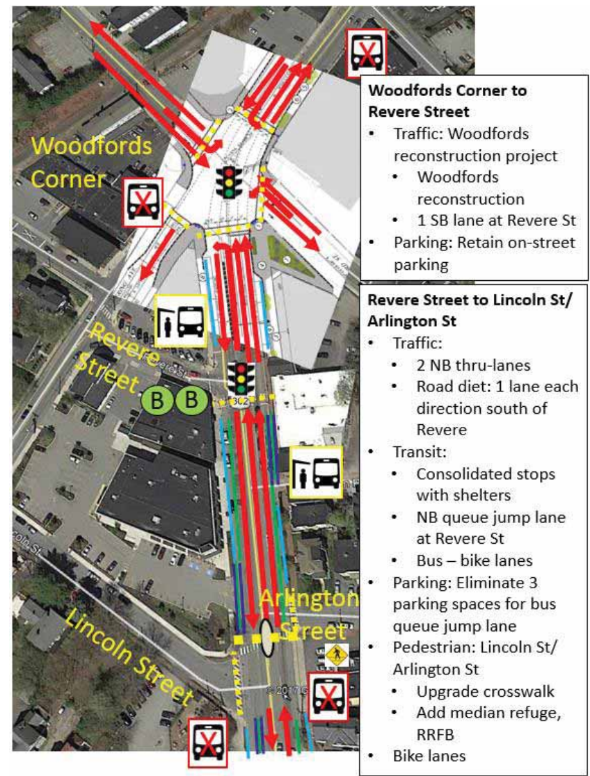
Figure 76. Woodfords Corner to Lincoln Street/Arlington Street – Alternative 2
