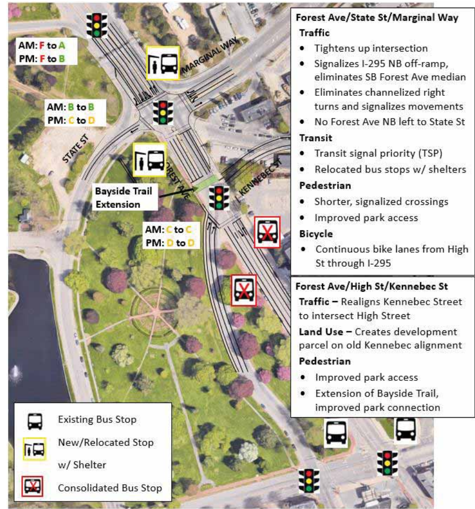
Figure 89. Deering Oaks Park – Alternative 2
