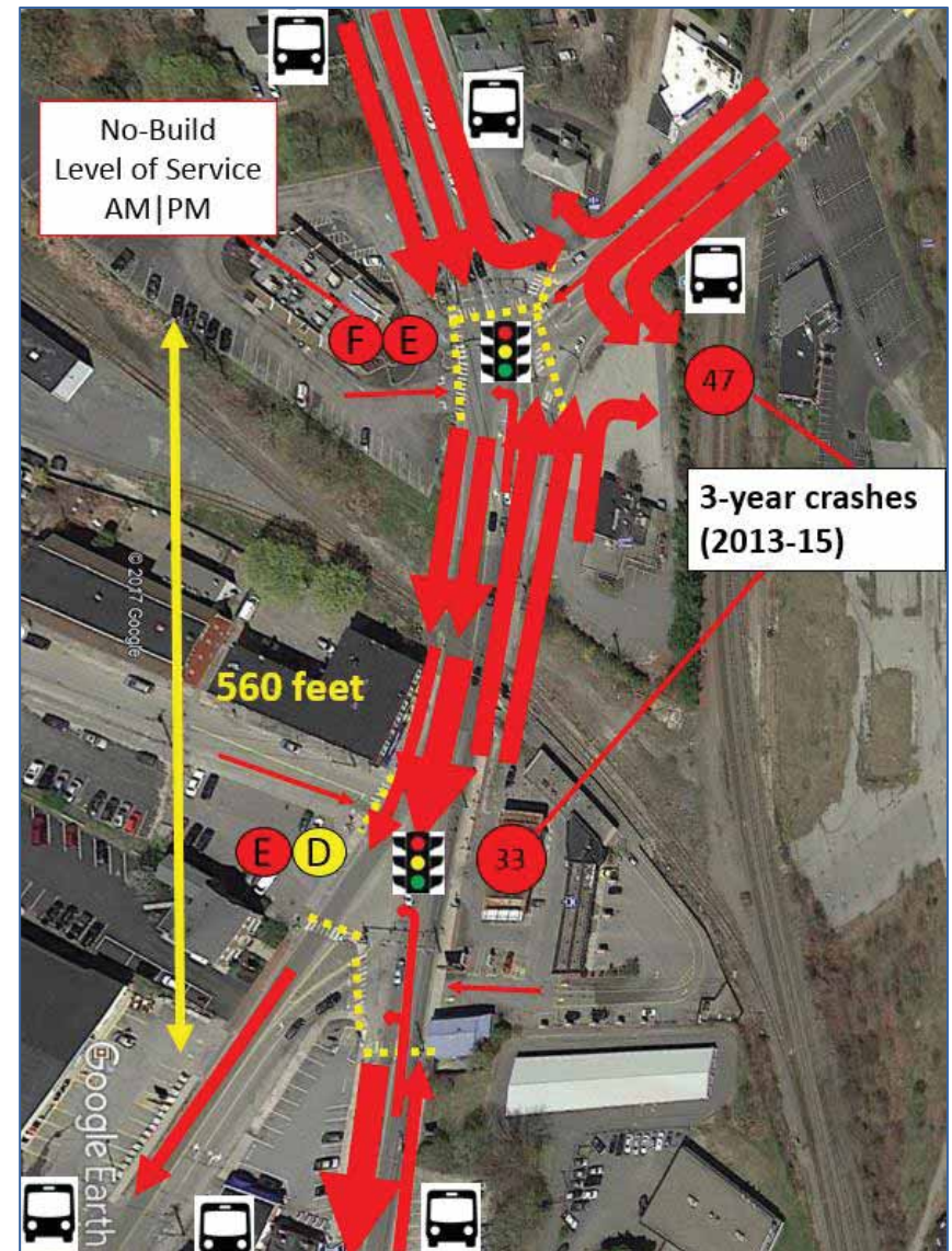
Figure 71. Morrill's Corner - Existing/No-Build Condition
