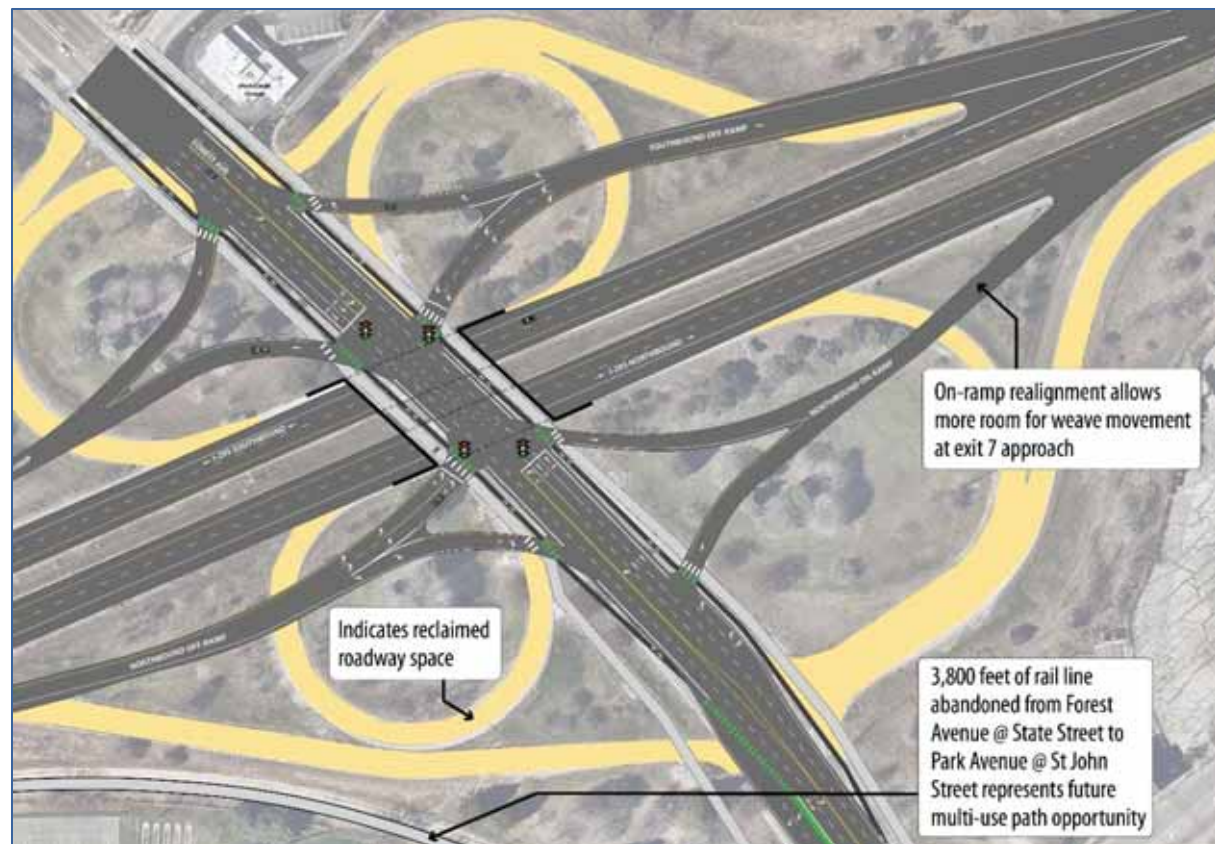
Figure 119. Potential Interchange Improvement – Redesign of I-295 Interchange, Exit 6 at Forest Avenue
