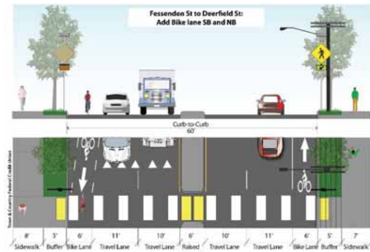
Figure 116. Alternative 1 — Forest Avenue from Deerfield Road to Fessenden Street
