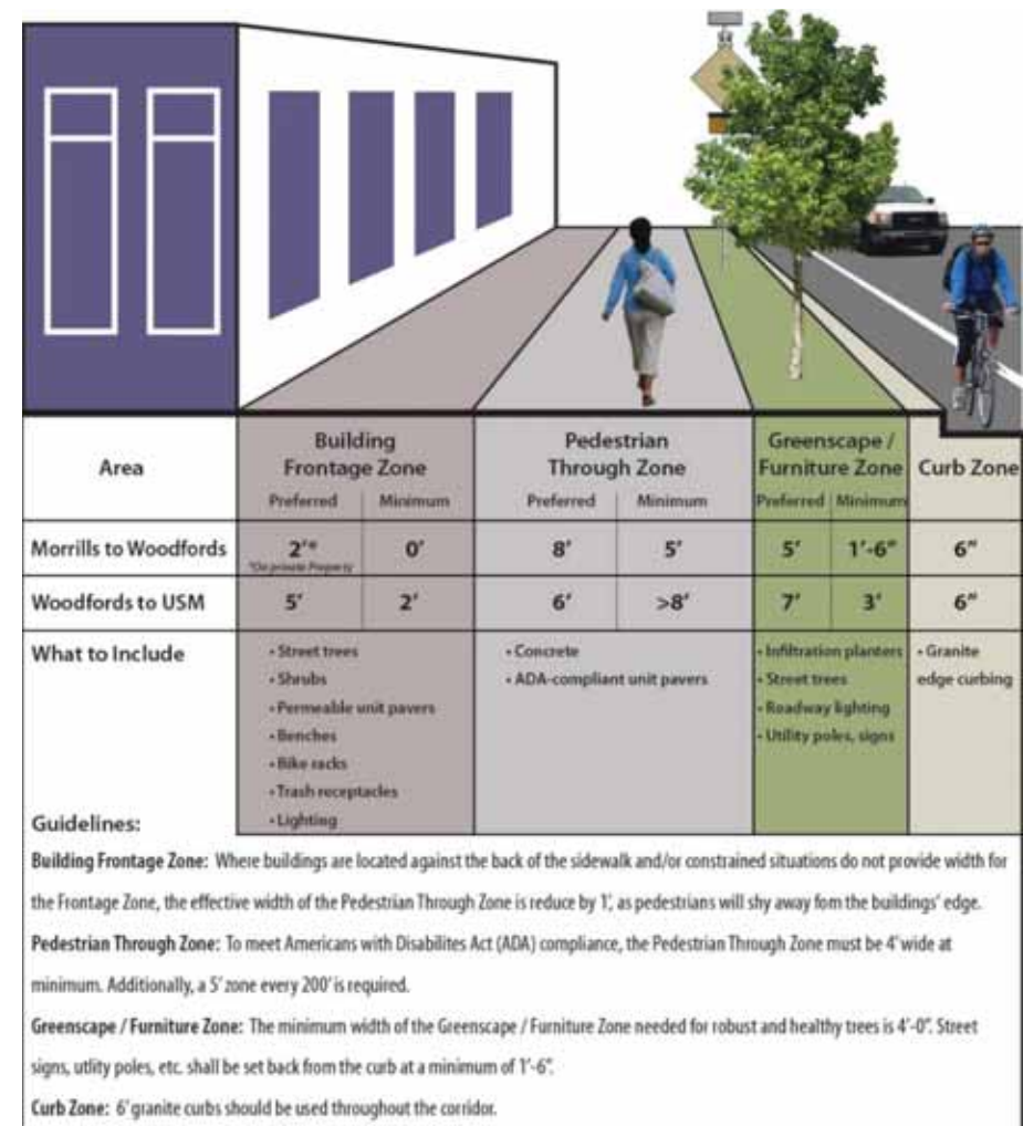
Figure 13. Public Realm Zones and Urban Design Guidelines
