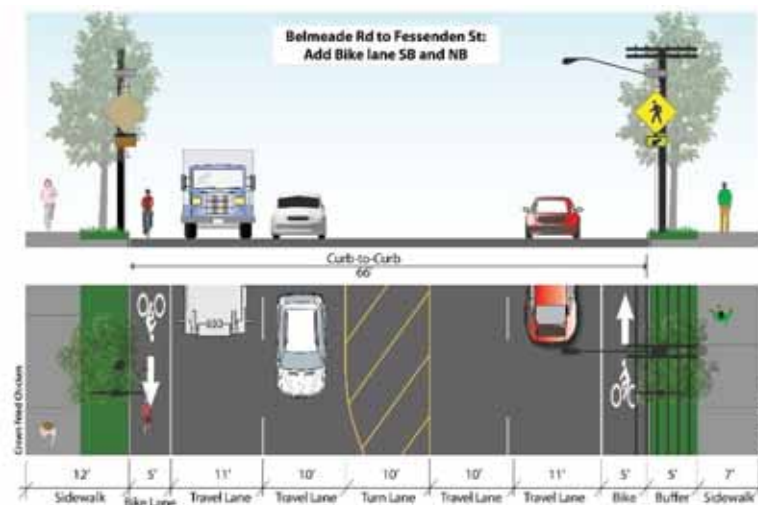
Figure 117. Alternative 1 — Fessenden Street to Belmeade Road
