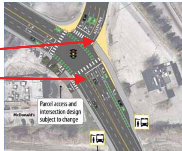
Figure 107. Variation on Preferred Alternative with Revised Property Access and Plaza Space at Northeast Corner of Forest Avenue and Allen Avenue
