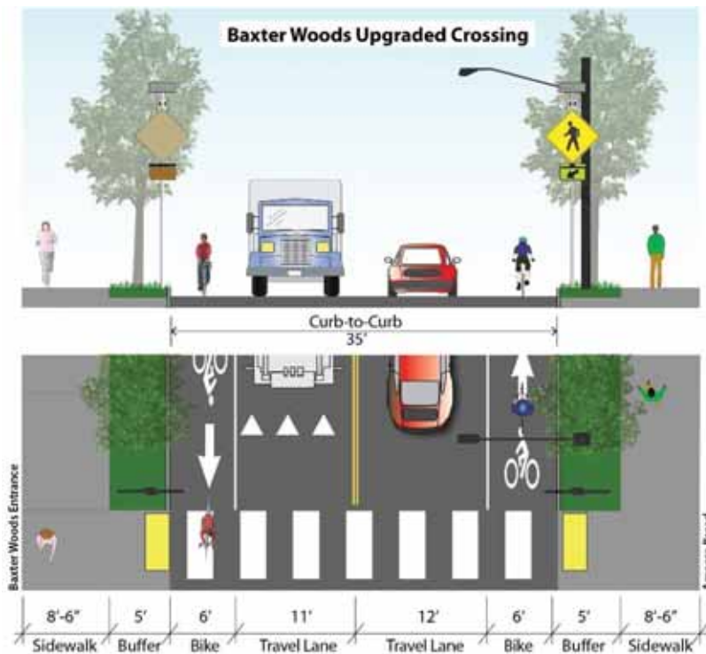
Figure 5. Upgraded Crosswalk with Rectangular Rapid Flashing Beacon and Pedestrian Neckdowns at Entry to Baxter Woods
