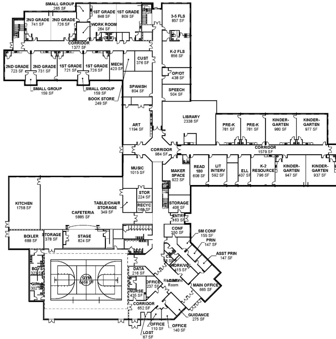
1 FIRST FLOOR PLAN A REVISION SCALE: 1/16" = 1'-0"
