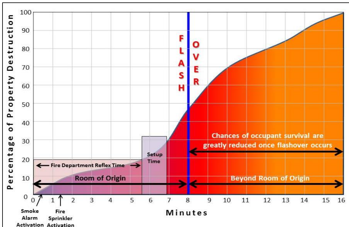
Figure 1. Fire Propagation Curve
